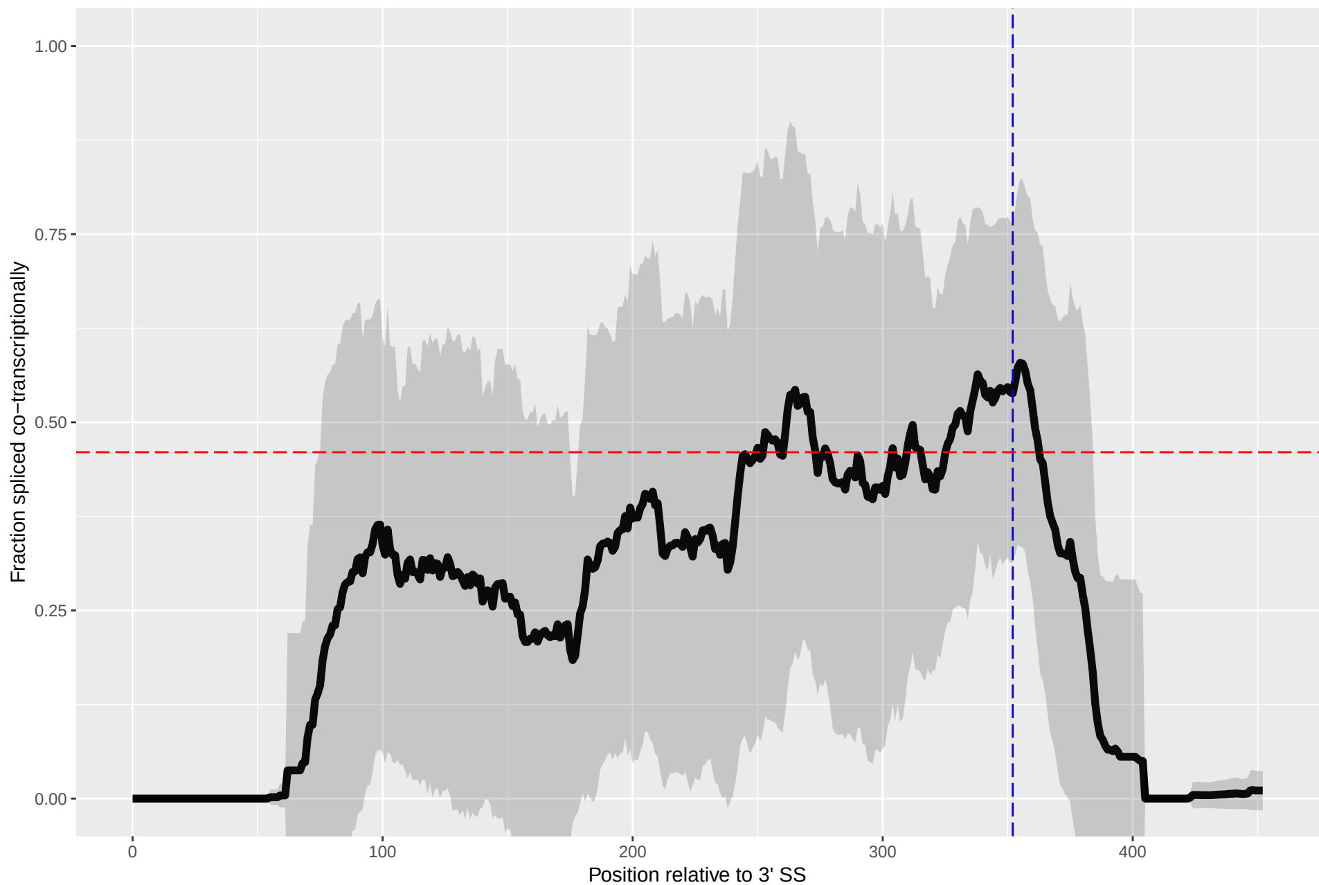
Splicing Kinetics for YKR095W-A
