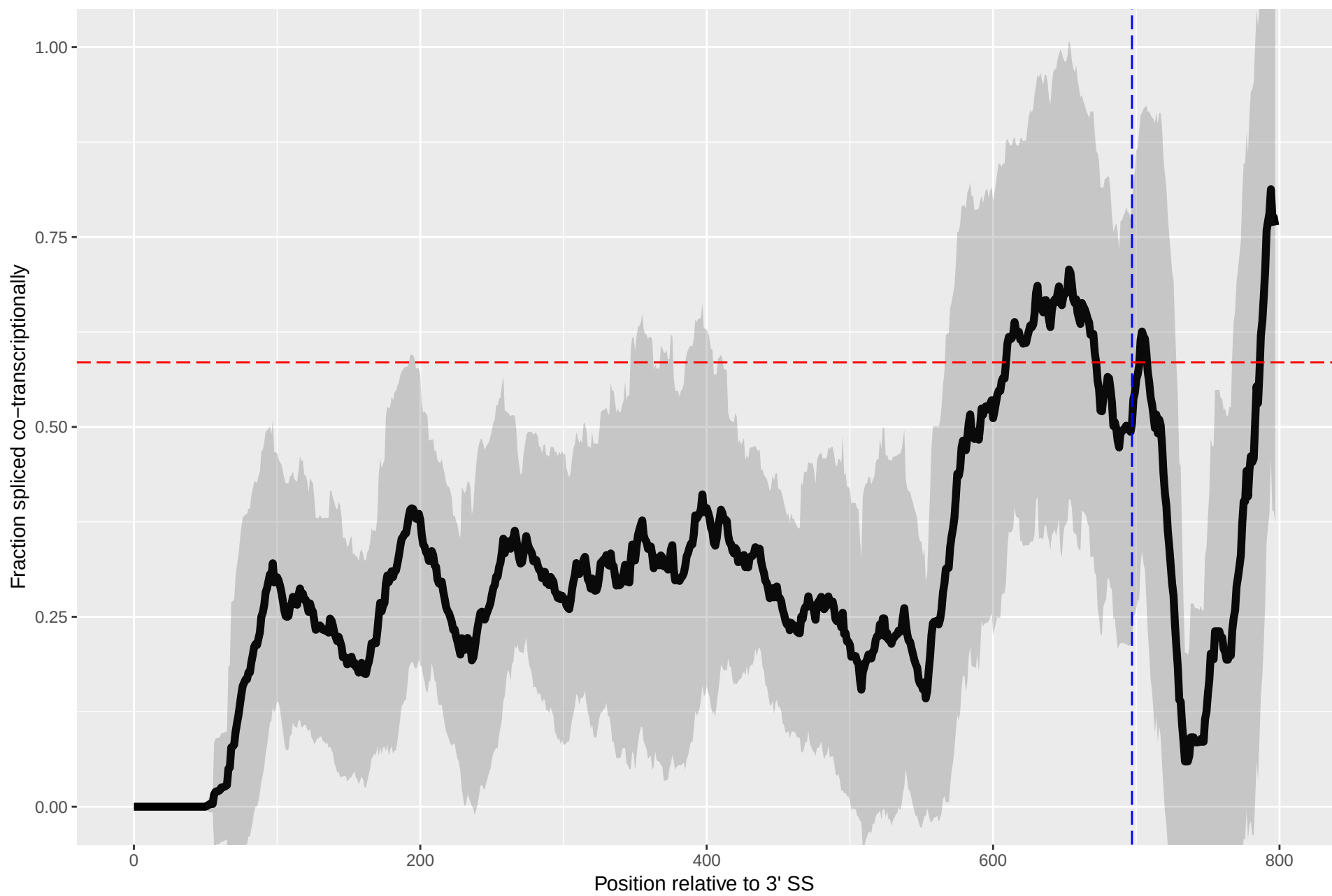
Splicing Kinetics for YJL001W
