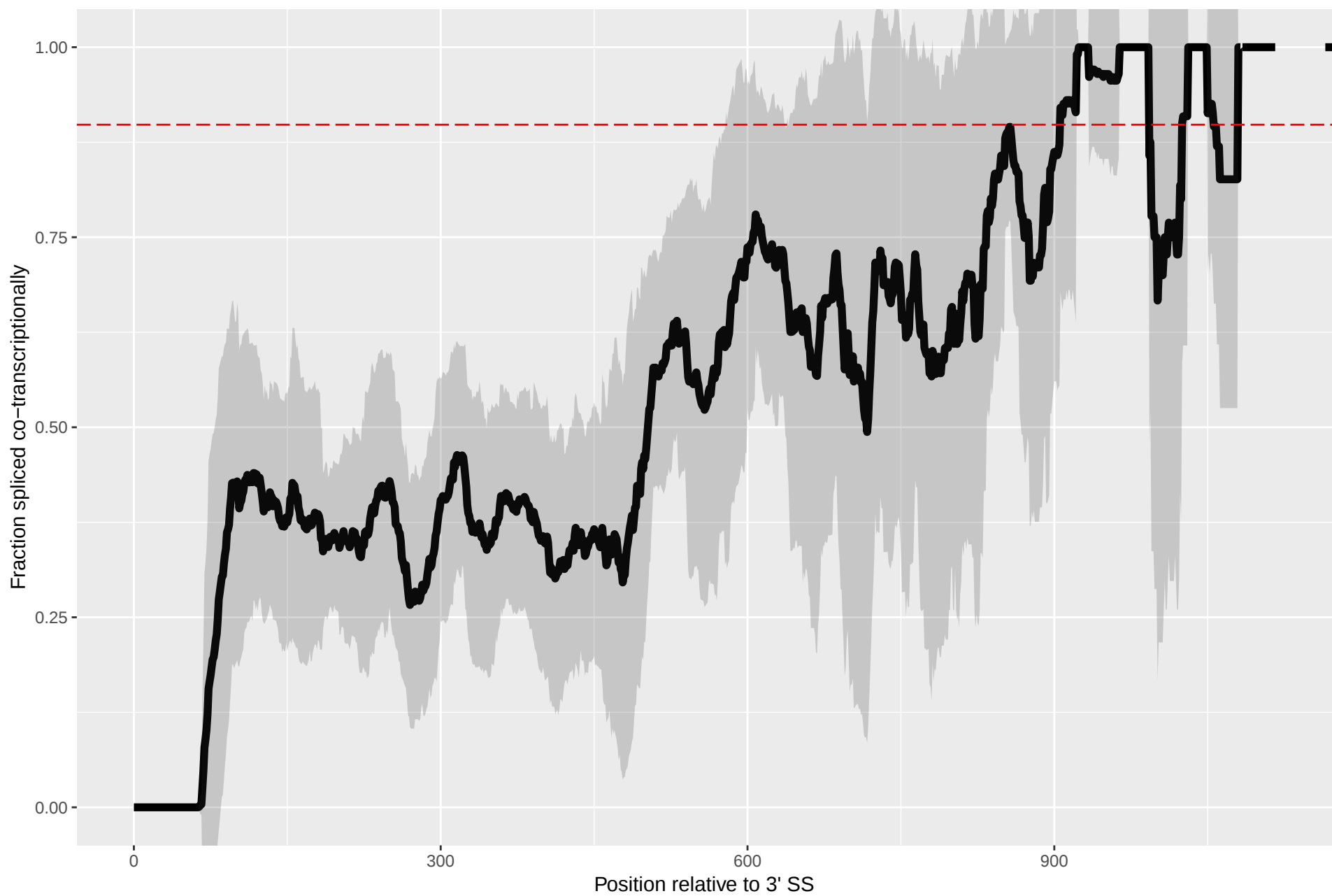
Splicing Kinetics for YGL137W
