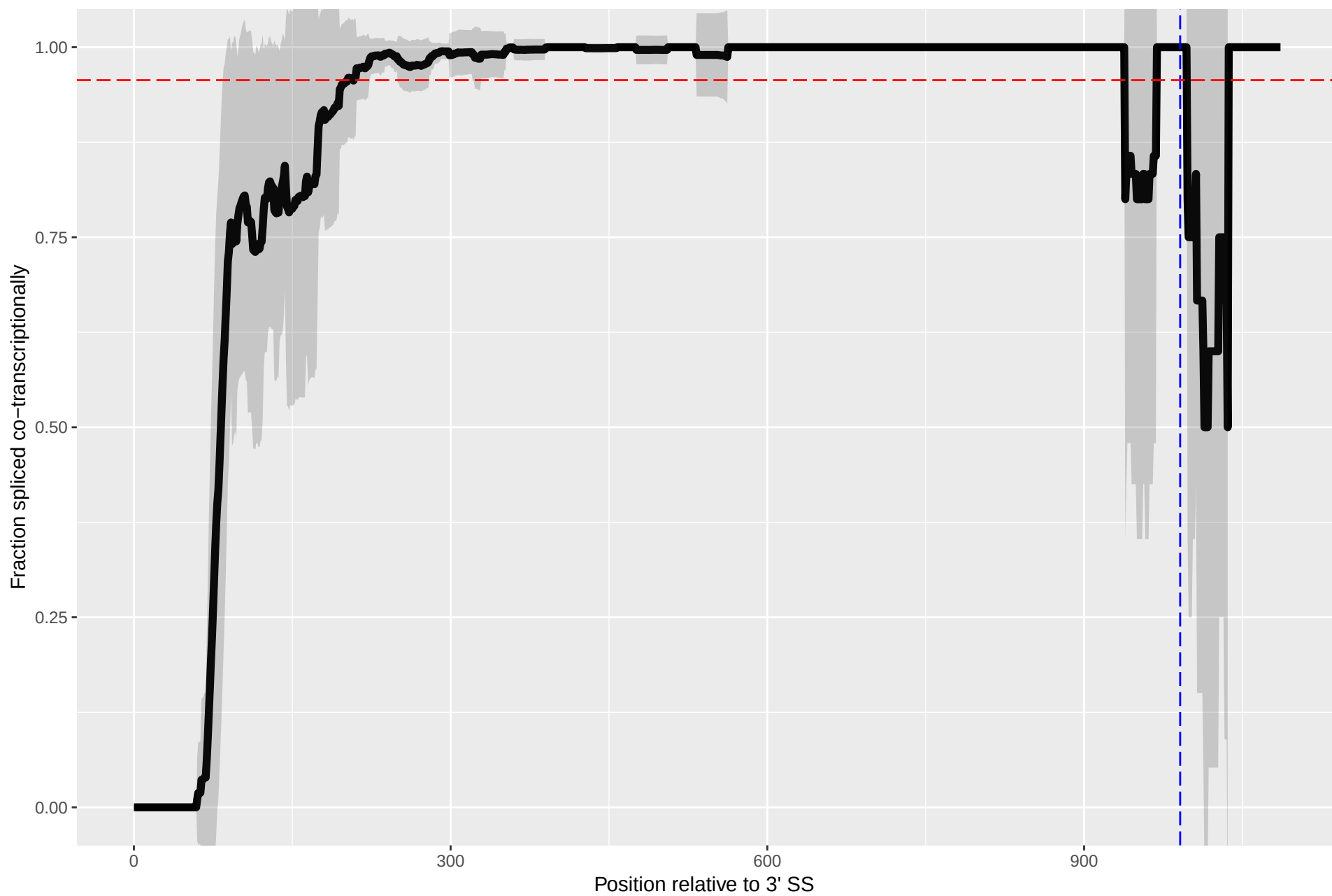
Splicing Kinetics for YER133W
