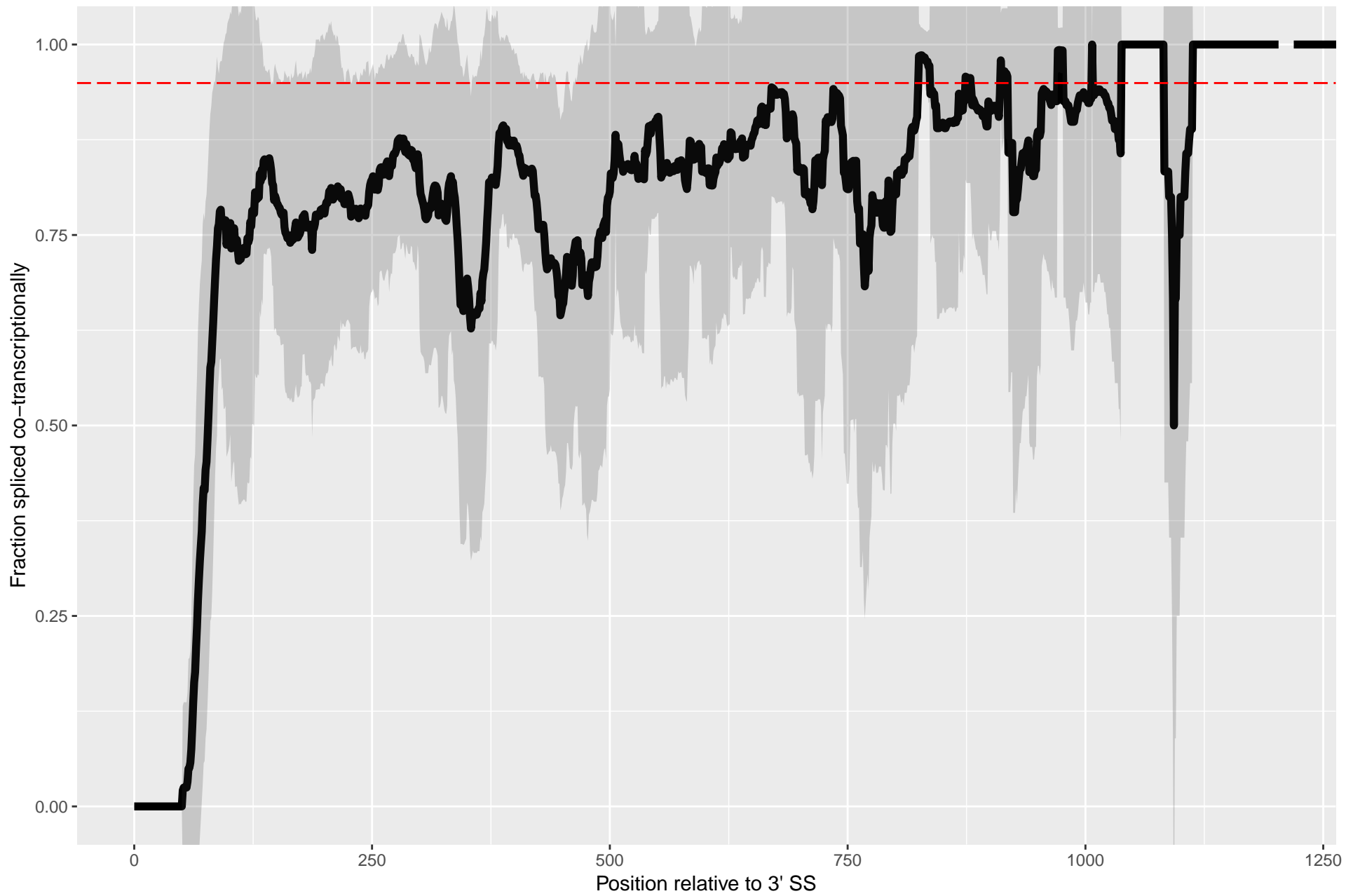
Splicing Kinetics for YJL041W
