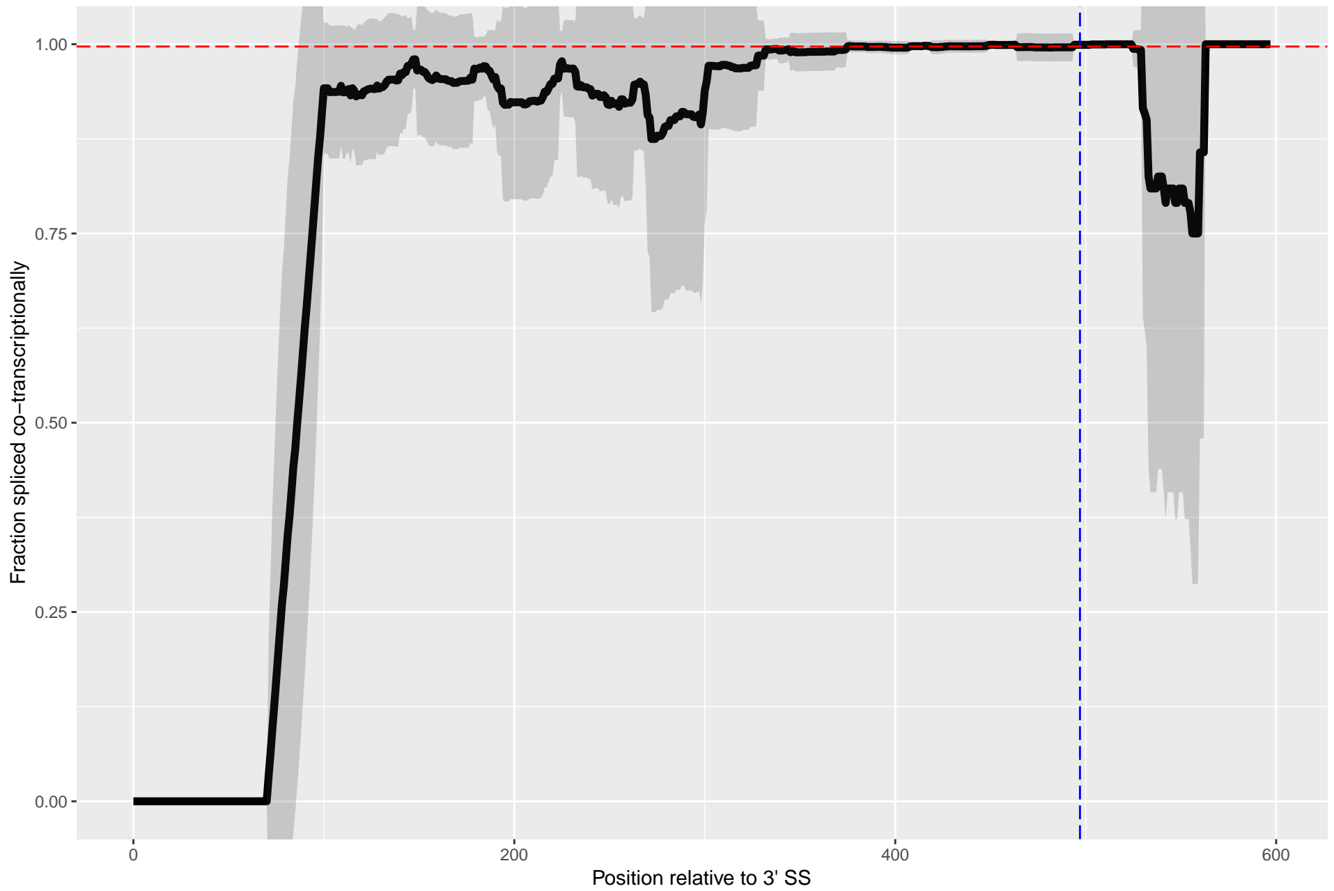
Splicing Kinetics for YDL136W
