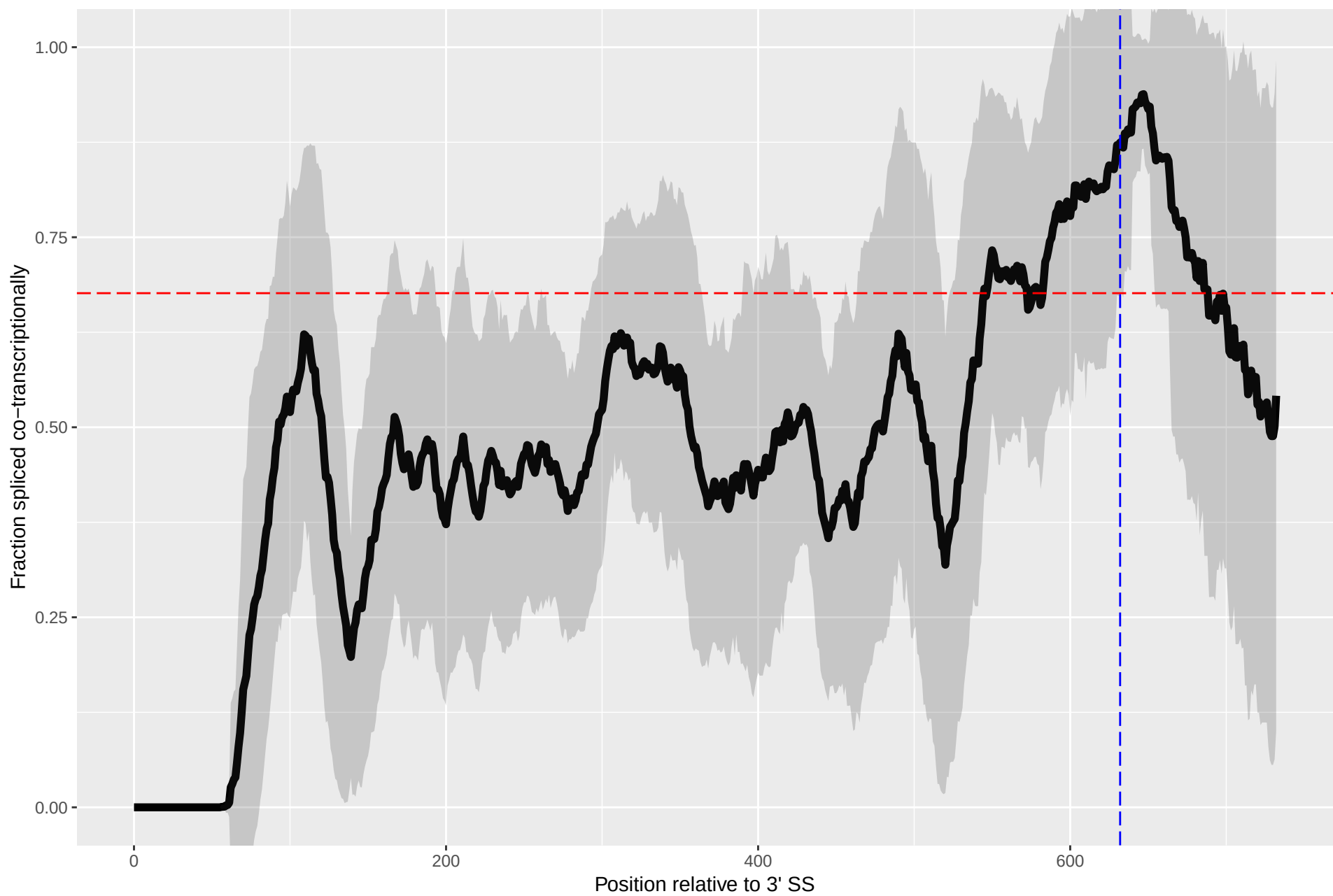
Splicing Kinetics for YPR028W
