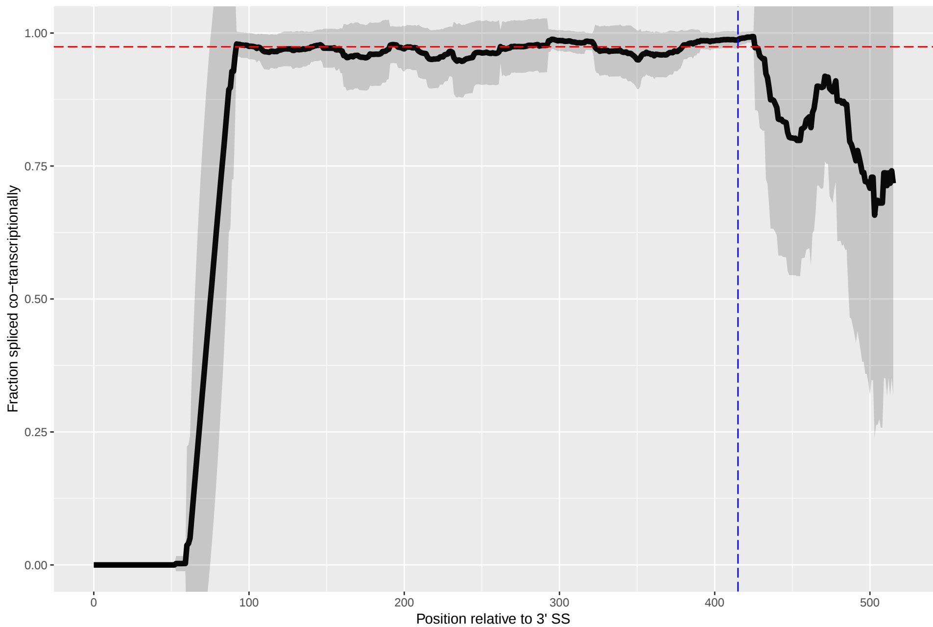
Splicing Kinetics for YGL030W
