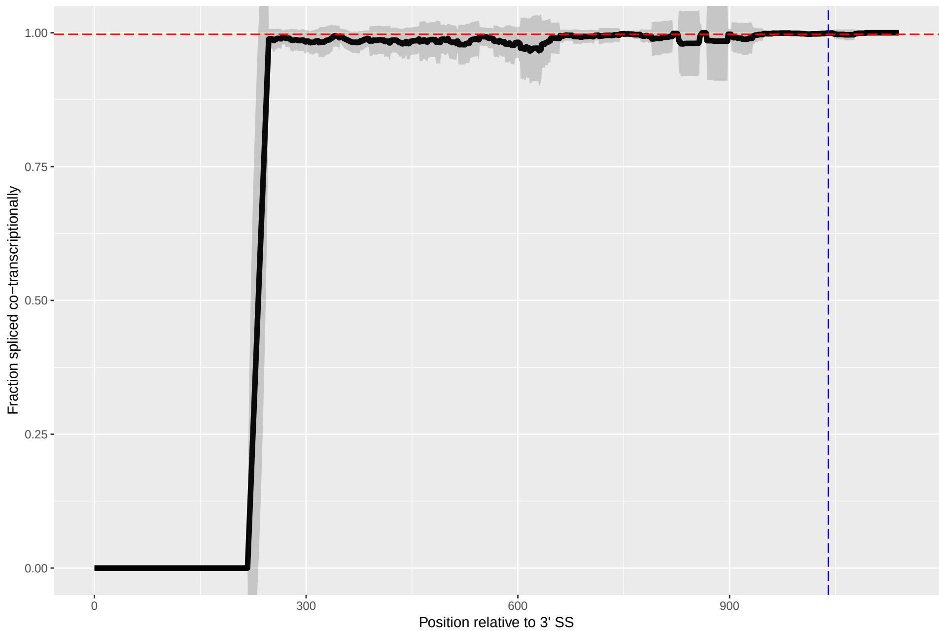
Splicing Kinetics for YFR031C-A
