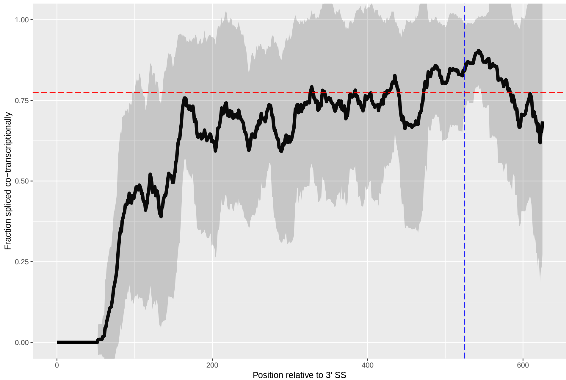
Splicing Kinetics for YDL064W
