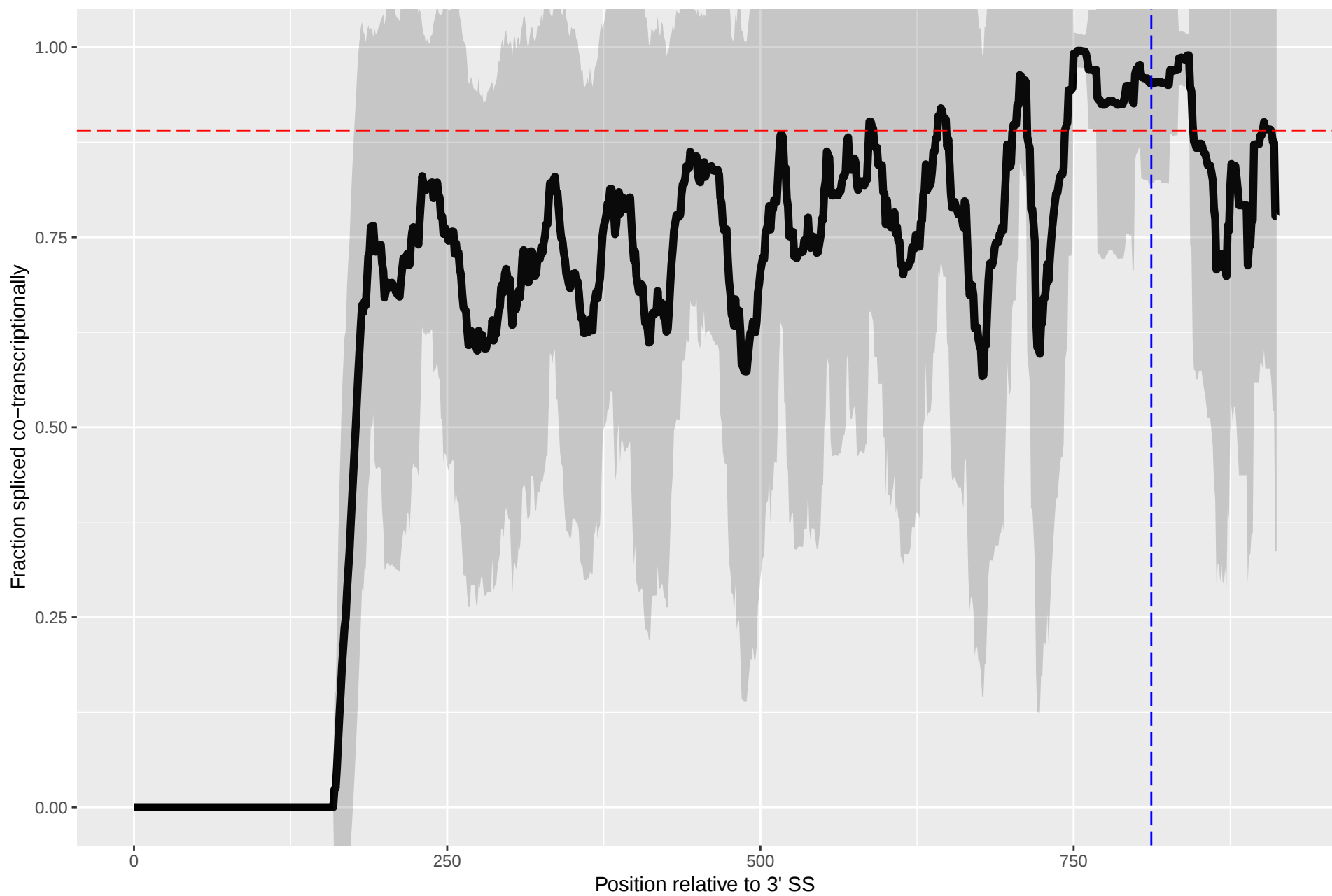
Splicing Kinetics for YBL040C
