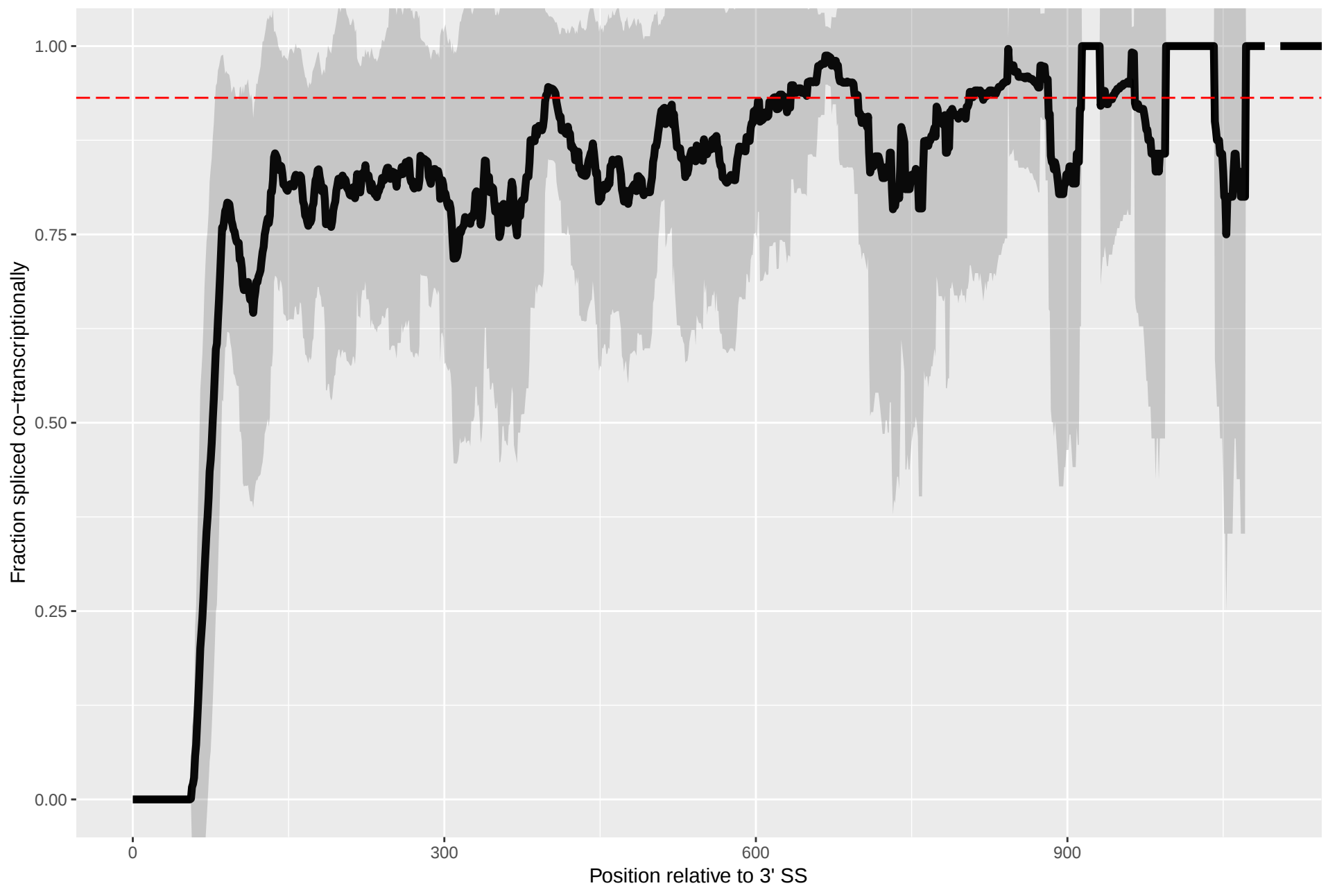
Splicing Kinetics for YJL041W
