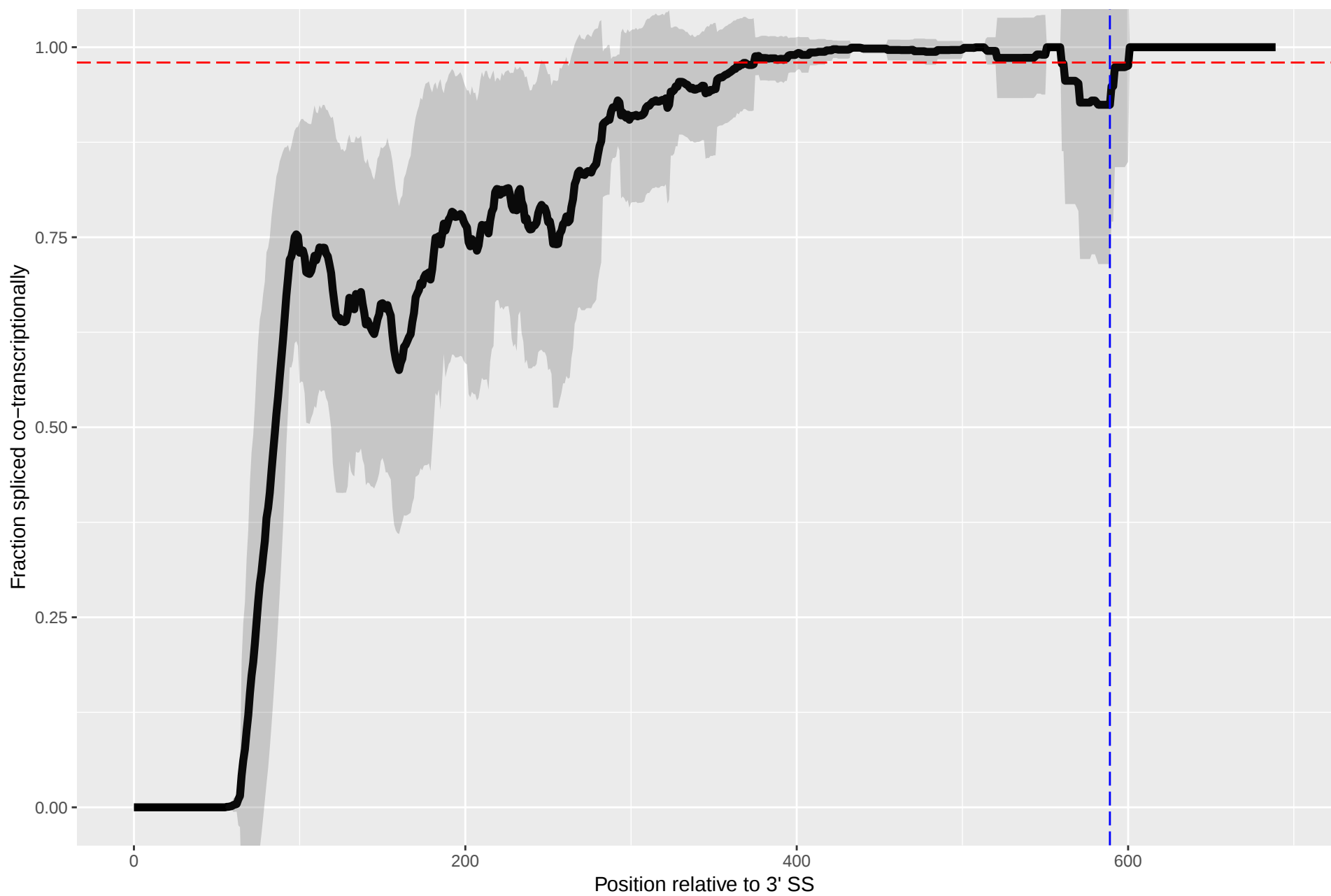
Splicing Kinetics for YDR381W
