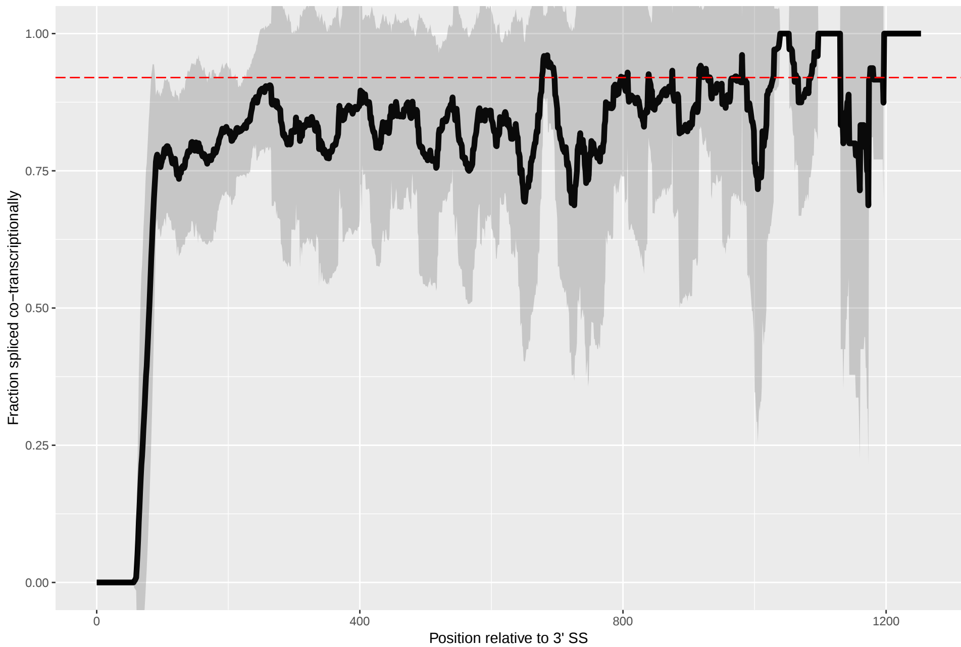
Splicing Kinetics for YMR033W
